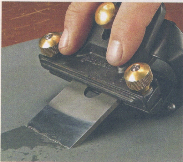
◀ A Sharp Edge. A honing guide ensures a consistent cutting angle and square edge.
