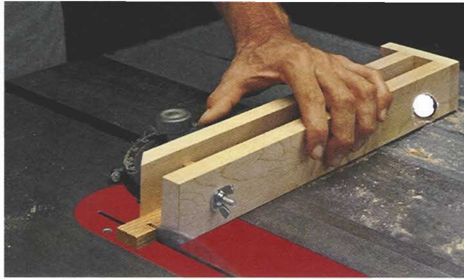
▲ Tight Between The Jaws. The jaws of the clamp can tightly grip even the smallest workpiece and keep your hands at a safe distance.
