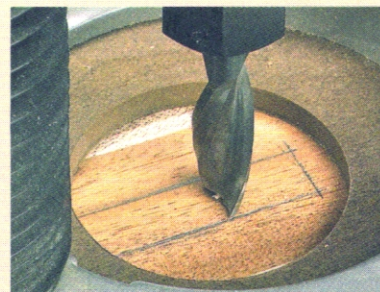
▲ Centering the Bit. Lower the bit to the surface and then reposition the jig to center it on the layout.
