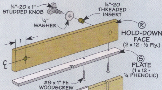
▲ Position Hold-Down. Set the hold-down on the workpiece and align the notch with the edge of the bit. Then lock the hold-down in place.
