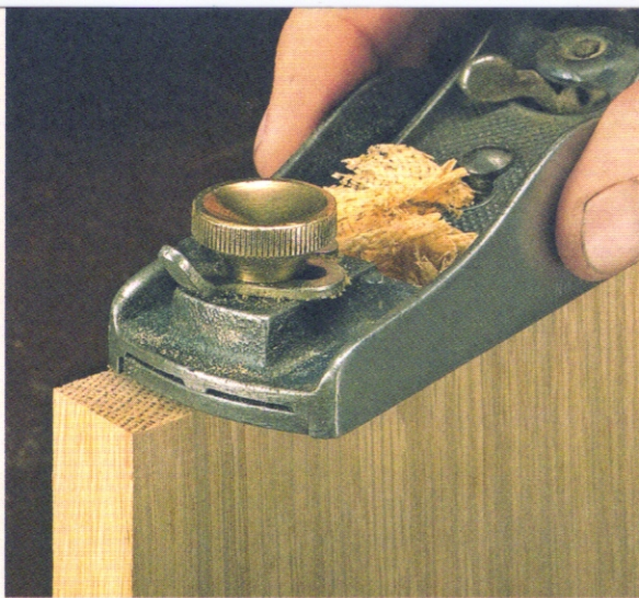
▲ A Tough Test. Shaving the end grain of a workpiece requires a keen cutting edge. As the edge dulls, the plane “chatters” and can’t make a clean shaving.
