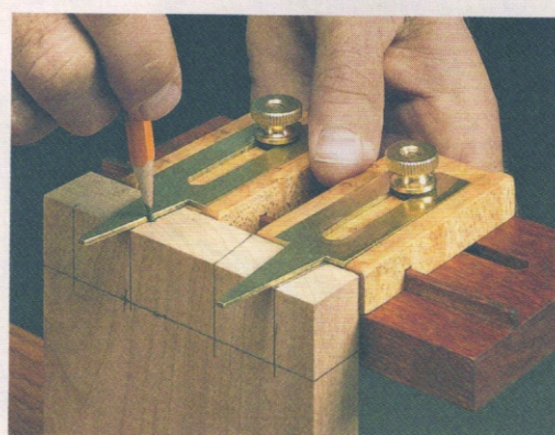
▲ Dovetail Layout. The angled dovetail keys make quick work of spacing and marking the pins of hand-cut dovetail joints.
