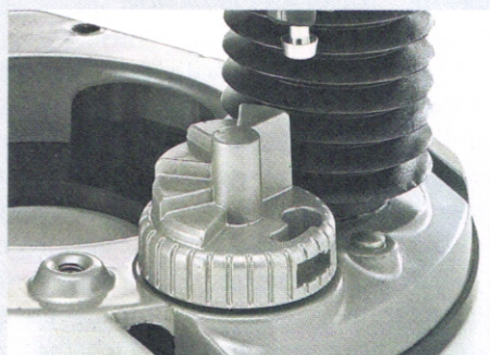
▲ Stepped Depth Stop. The steps of this rotating "turret" stop let you quickly make a cut in several passes.
