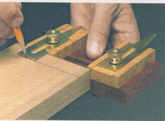
▲ Scribing Lines. A small notch in the end of each key holds your pencil tip for marking lines parallel to the edge of a workpiece.
